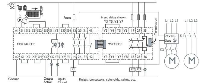
115V/230V AC Supply, 24V DC, Dual Channel, Automatic Reset, Monitored Output
