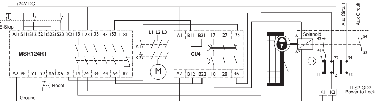
Single Channel Wiring to CU4 Inputs
