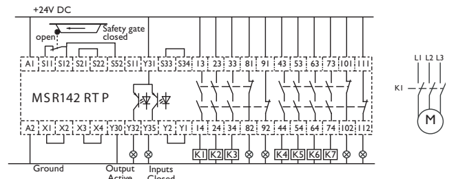
Single Channel Safety Gate, Auto Reset, No Output Monitoring
