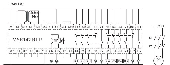
Safety Mat, Automatic Reset, No Output Monitoring
