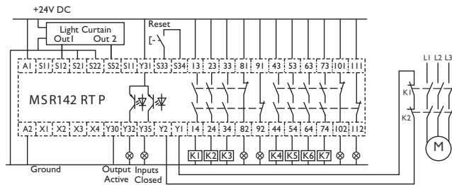
Light Curtain, Monitored Manual Reset, Monitored Output
