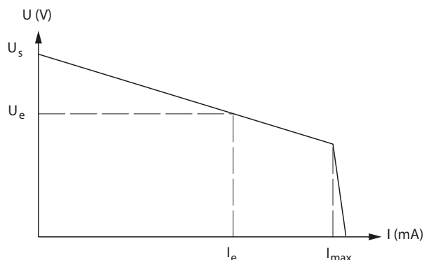
Output characteristics
