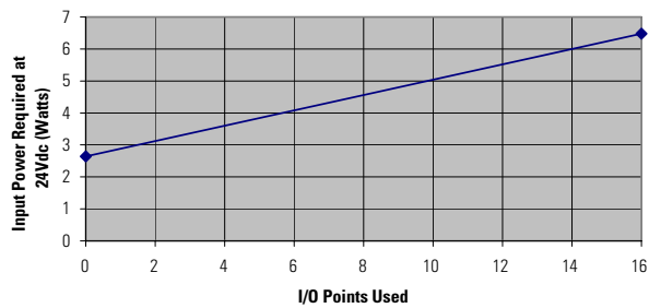
1761-L16BWB Typical Power Requirements
