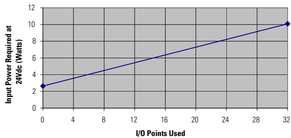
1761-L32BWB Typical Power Requirements
