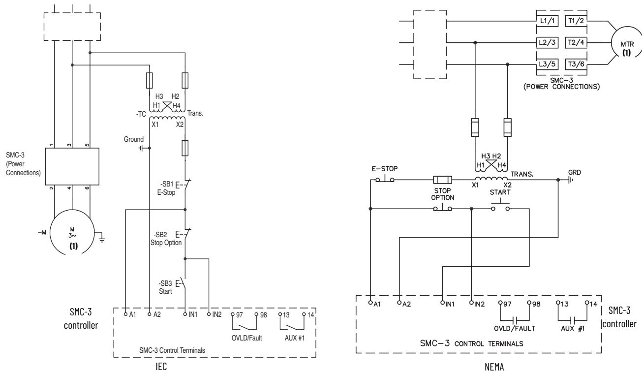
Figure 2 - Three-wire Configuration
