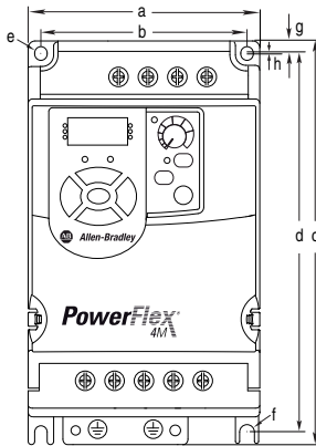
Figure B.1 PowerFlex 4M Panel Mount Drives
