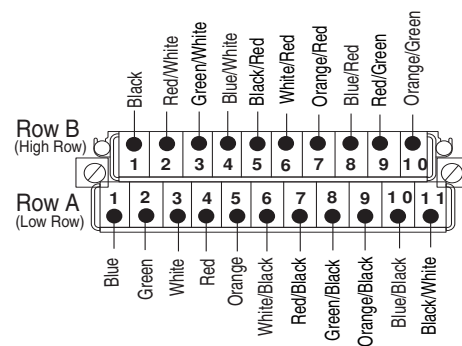
1492-CAB01U64
