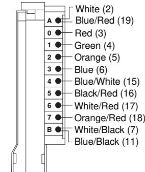
1492-CABLE 1T
