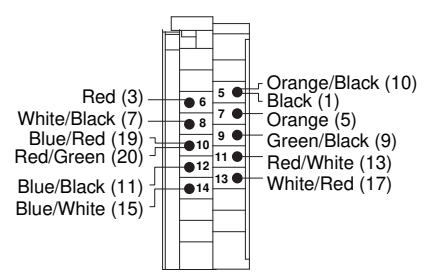
1492-CAB1C69
