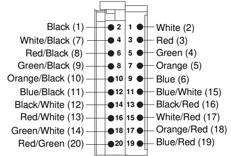
1492-CABLE 1U
