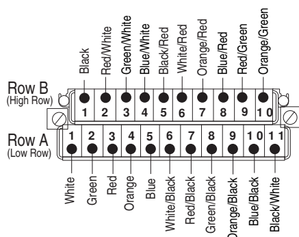
1492-CAB0T64
