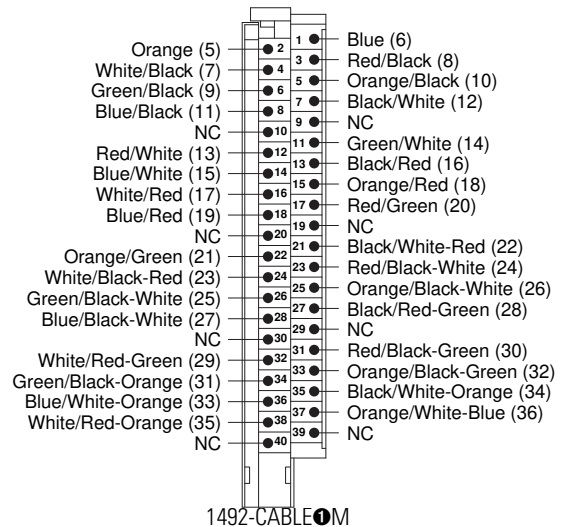
1492-CABLE M
