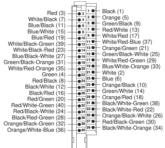
1492-CABLE K
