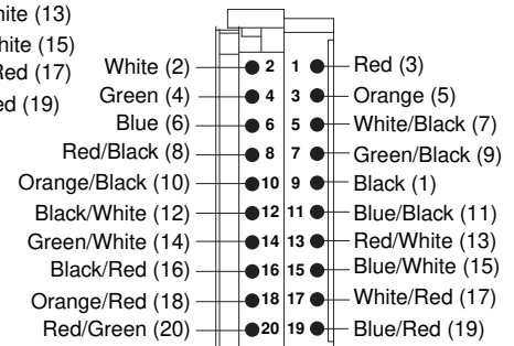
1492-CABLE 1W
