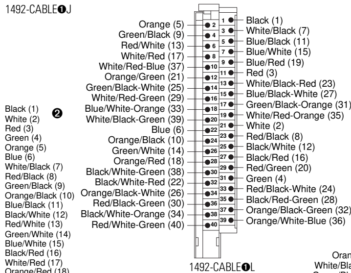
1492-CABLE L
