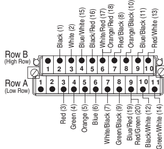
1492-CAB1C64
