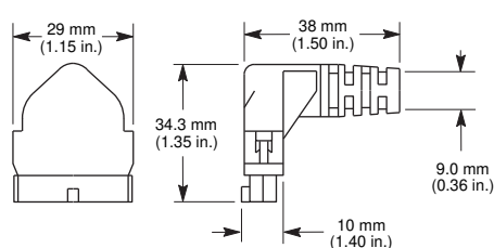
20-Point Cable Dimensions
