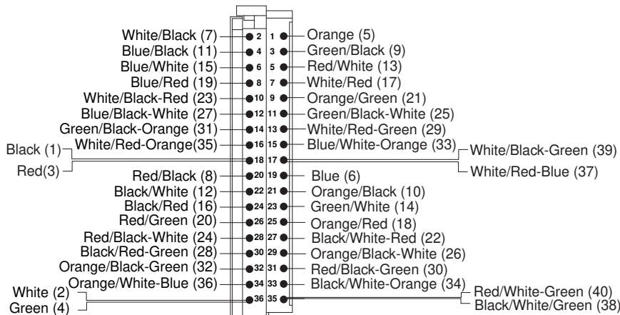
1492-CABLE 1X
