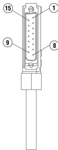
15-Pin D-Shell Connector
