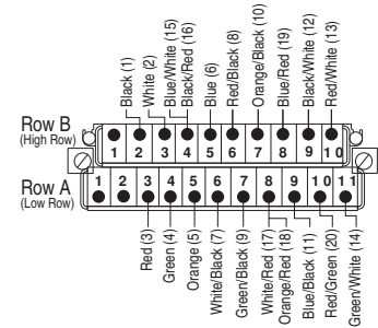
1492-CAB1F64
