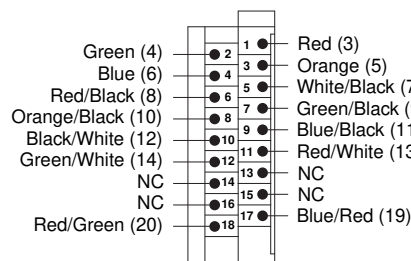
1492-CAB1G69
