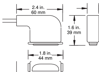
15-Pin D-Shell Dimensions
