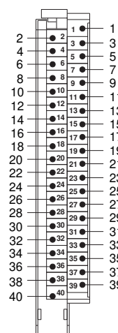
1492-CABLE0WBN
