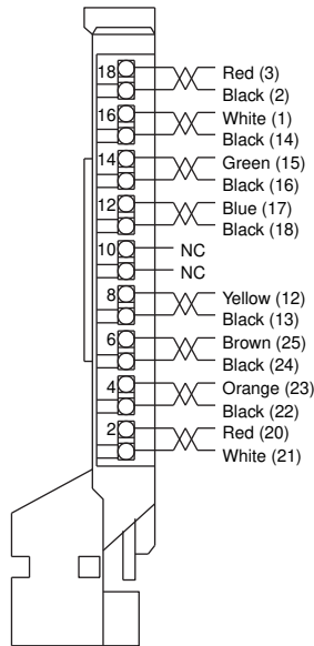
1492-ACABLE___H
