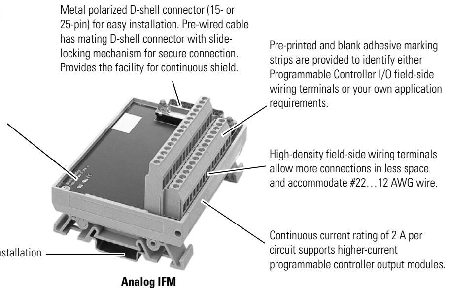
Analog IFM
