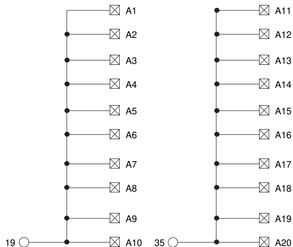
Blown Fuse Indicator Circuit
