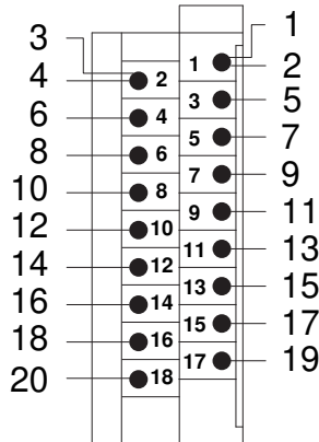
1492-CAB0RTN18
