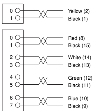
1492-ACABLE___B
