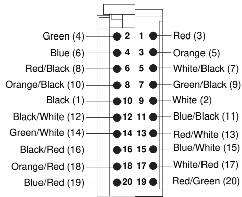
1492-CABLE 1X
