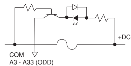
Blown Fuse Indicator Circuit
