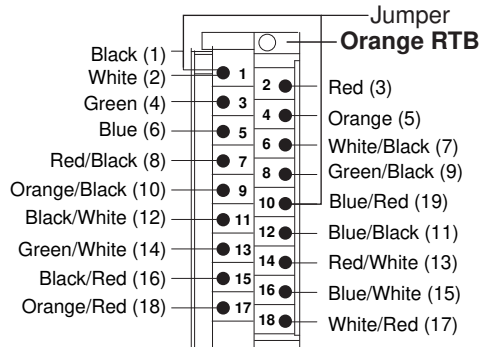
1492-CABLE 1N
