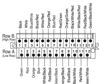
1492-CAB0T64
