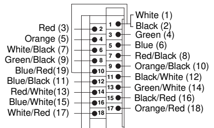
1492-CAB1H69
