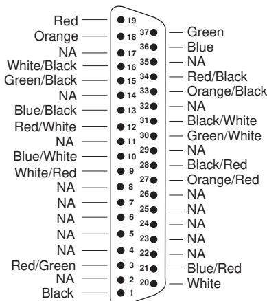
1492-CAB0G94 ③
