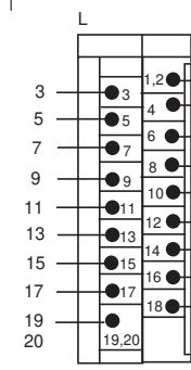
Cable Wiring Table Conductor for 1492-CAB0H94
