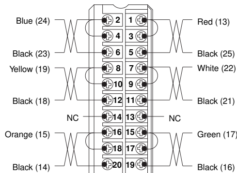
1492-ACABLE___X
