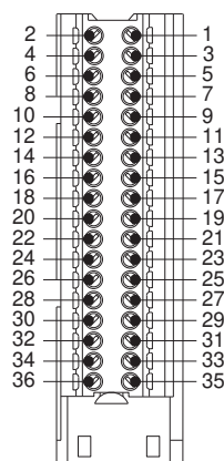
1492-CABLE0TBCH
