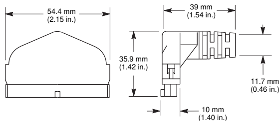
40-Point Cable Dimensions
