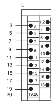
Cable Wiring Table Conductor for 1492-CAB0H94
