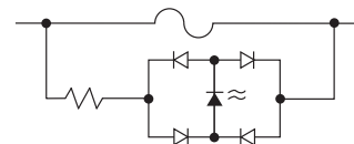
Blown Fuse Indicator Circuit
