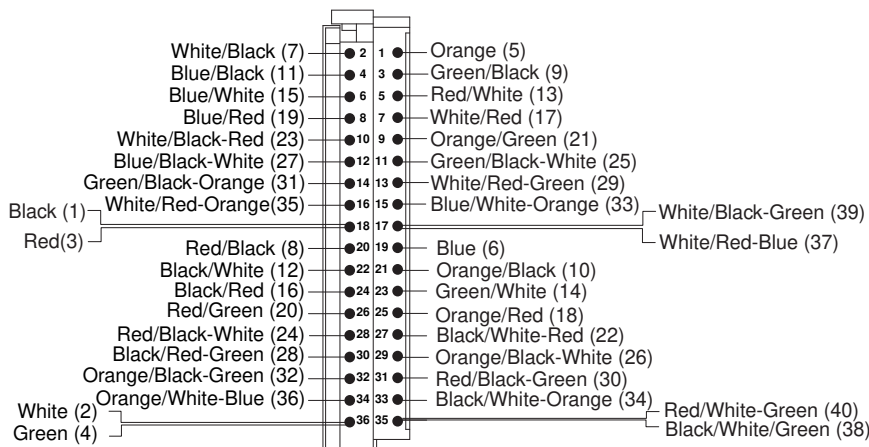
1492-CABLE 1X
