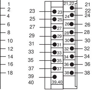
Cable Wiring Table Conductor for 1492-CAB0H94
