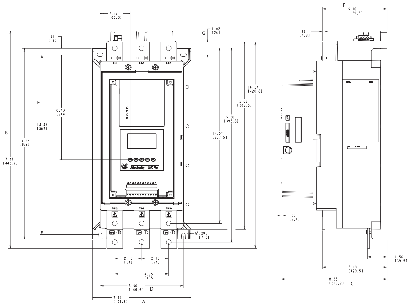
Figure 14 - 108...135 A Controllers
