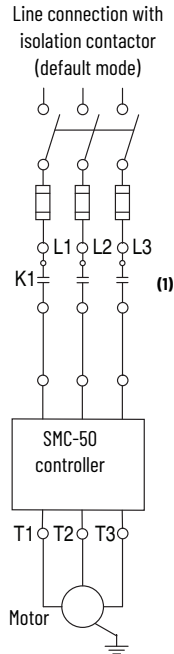
Figure 20 - Typical Power Wiring Diagrams
