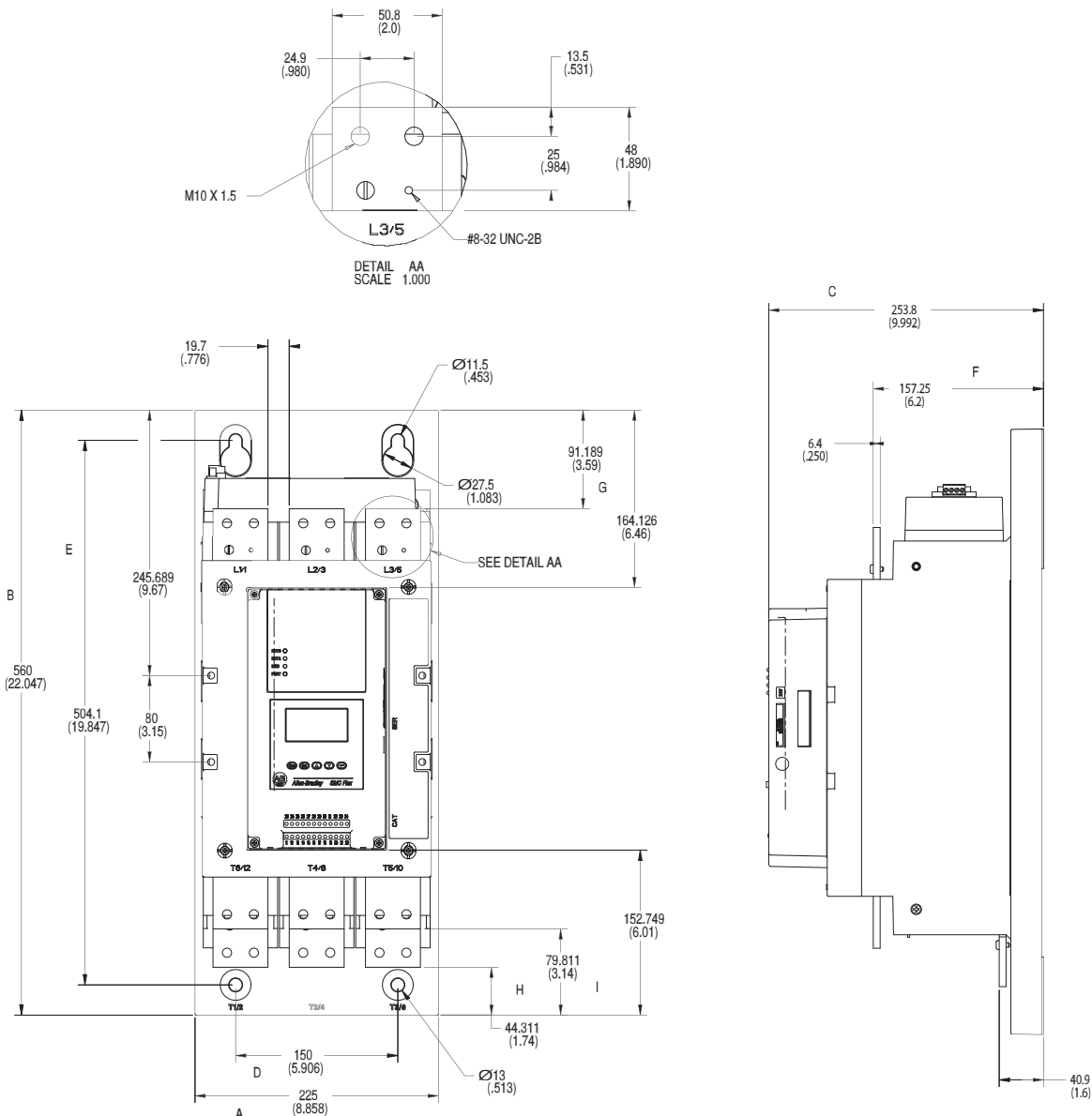
Figure 15 - 201...251 A Controllers
