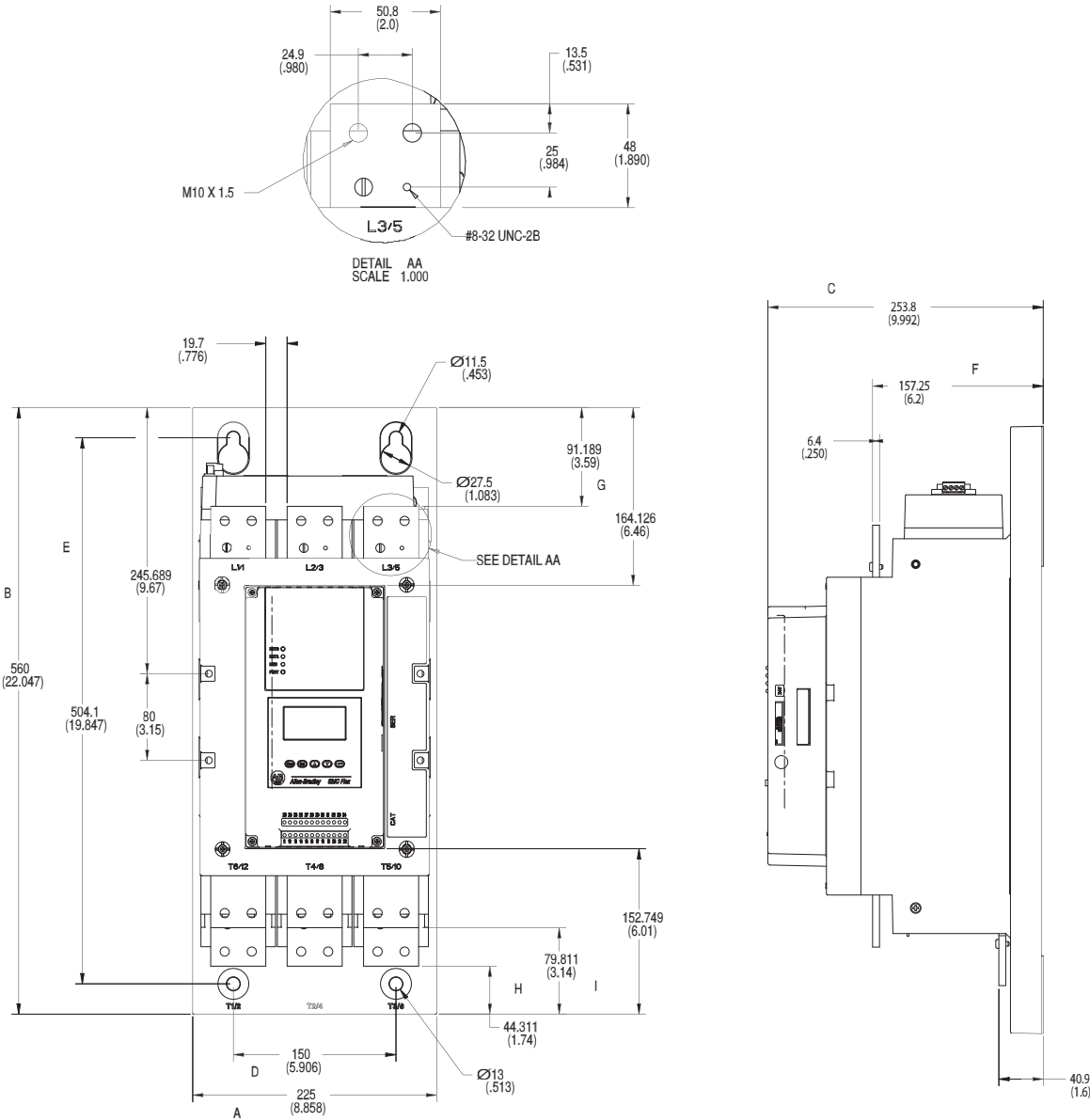
Figure 15 - 201...251 A Controllers
