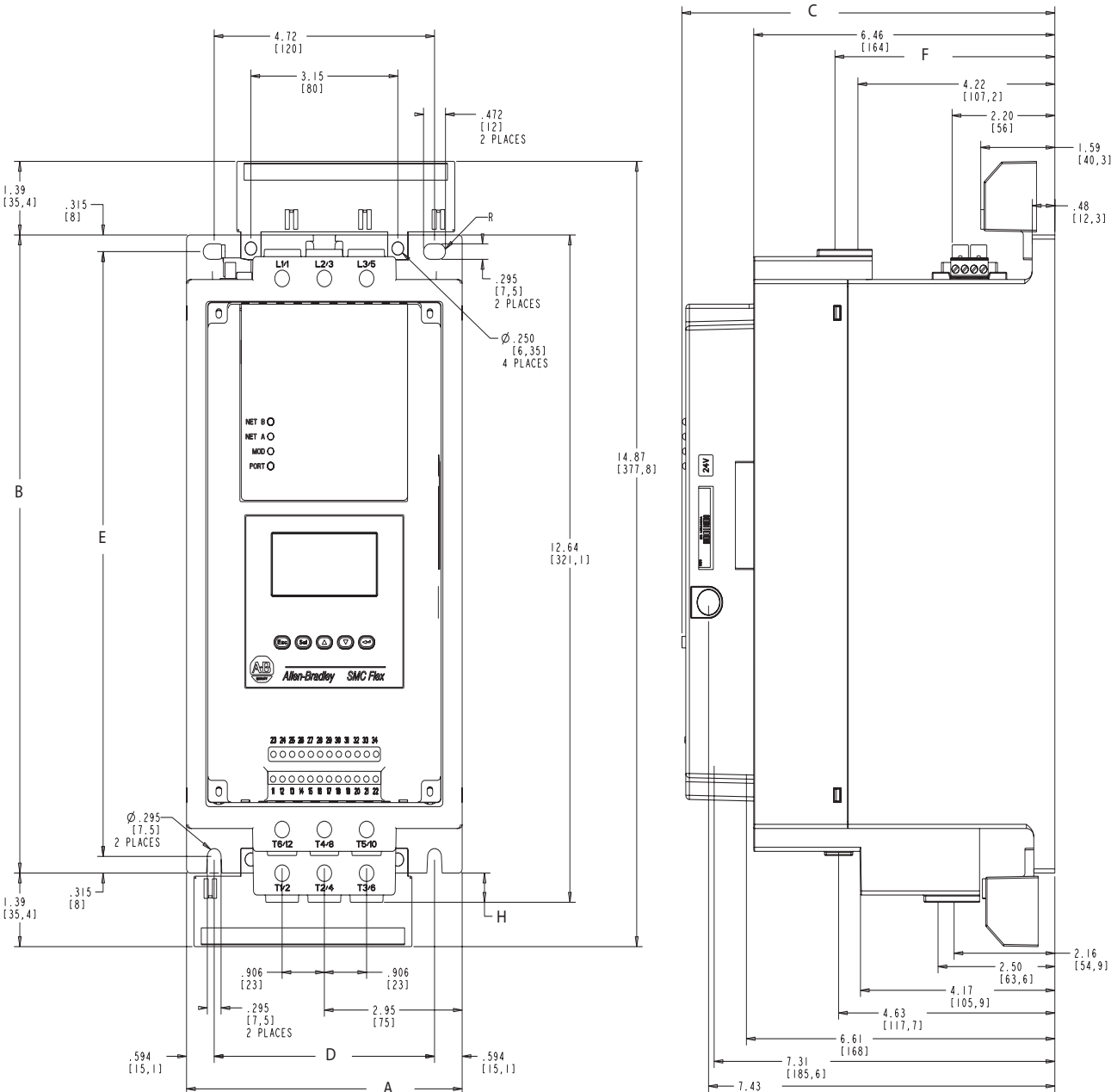
Figure 13 - 5...85 A Controllers
