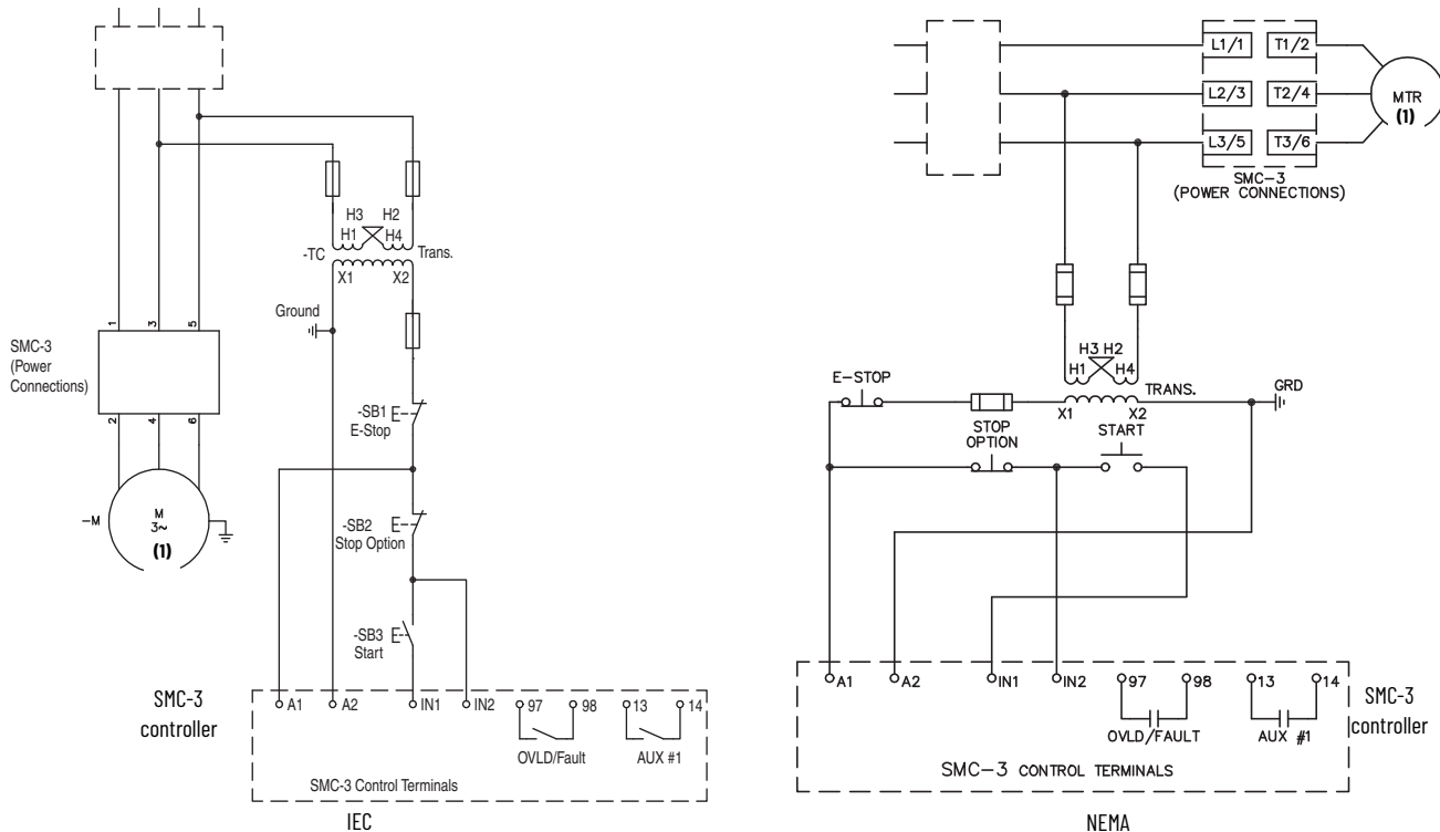
Figure 2 - Three-wire Configuration
