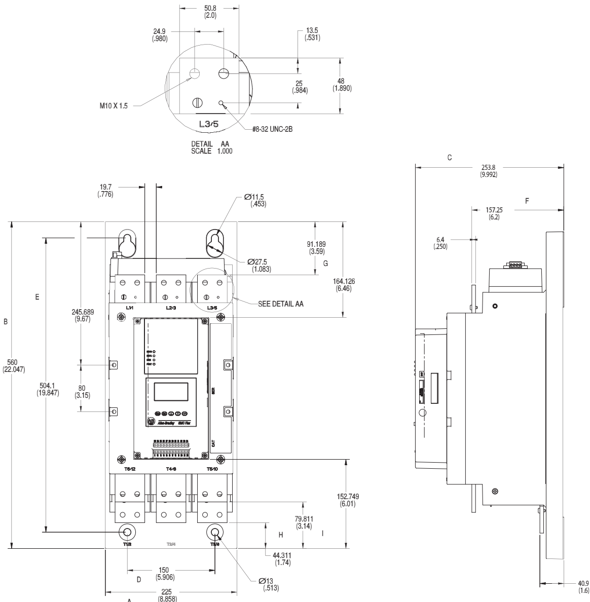
Figure 15 - 201...251 A Controllers
