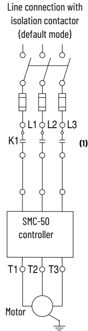
Figure 20 - Typical Power Wiring Diagrams
