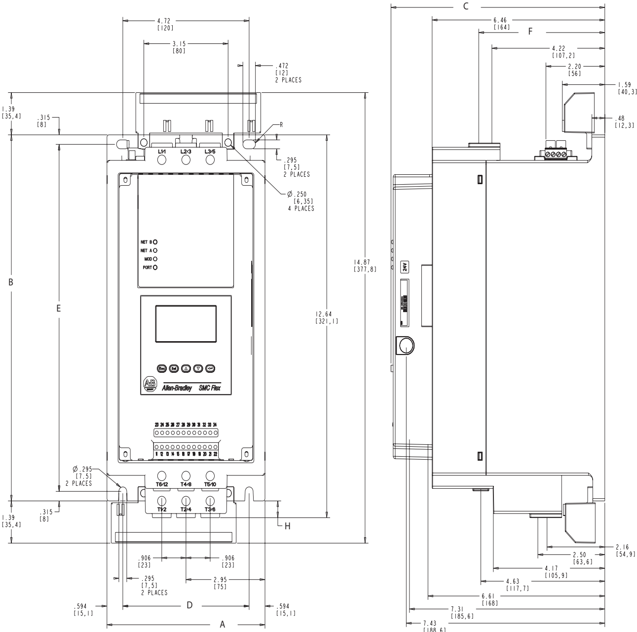
Figure 13 - 5...85 A Controllers
