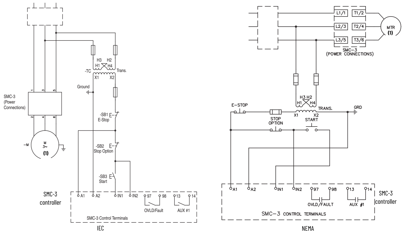
Figure 2 - Three-wire Configuration
