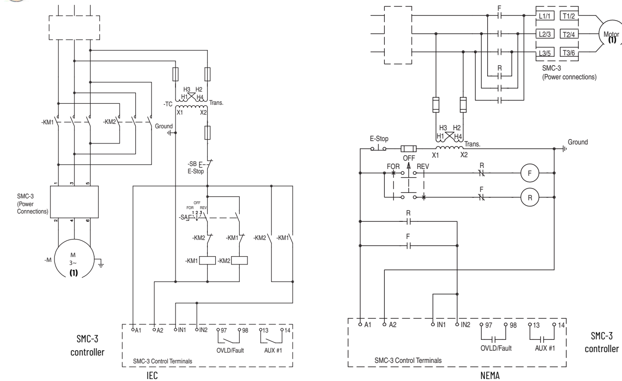
Figure 4 - Reversing Configuration
