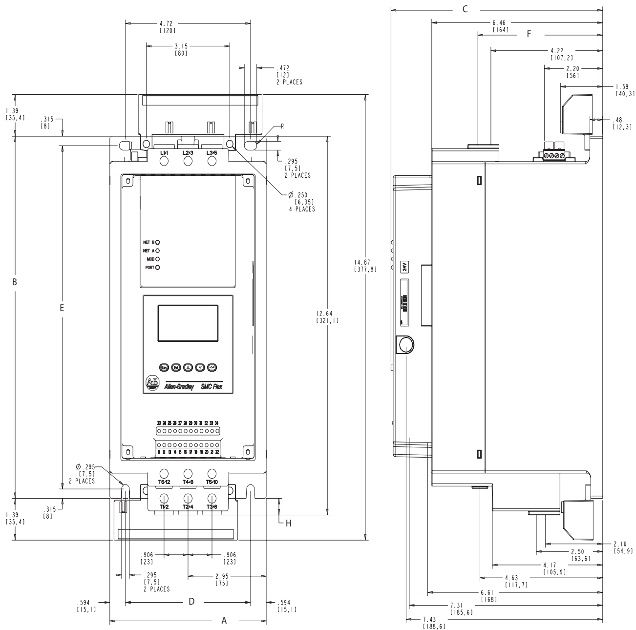
Figure 13 - 5...85 A Controllers
