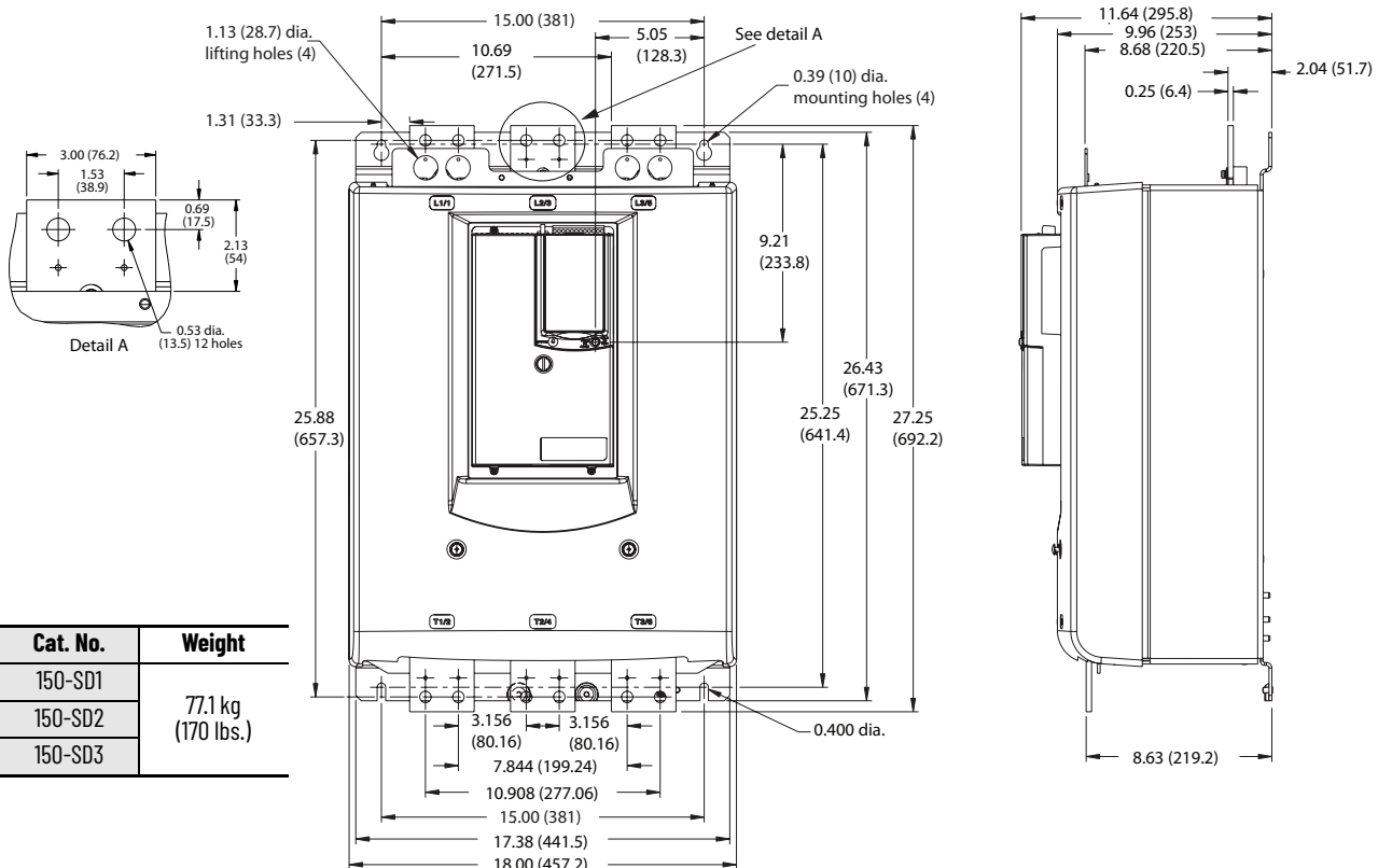
Figure 33 - Cat. Nos. 150-SD1...SD3 Solid-state Controller
