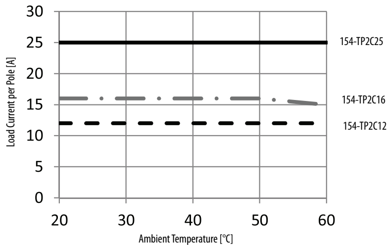
Figure 5 - Current Derating—Cat. No. 154-TP2...Devices
