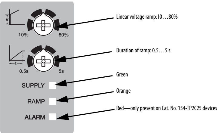
Figure 2 - Adjustment Dial
