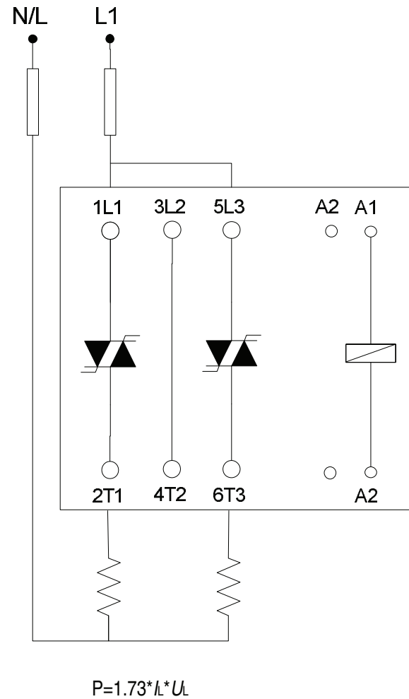
Figure 36 - Dual-phase Contactor, Line-Neutral/Line-Line Connection
