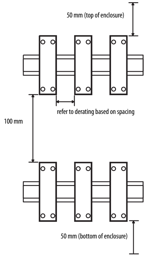
Recommended Contactor Spacings
