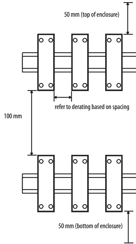
Recommended Contactor Spacings
