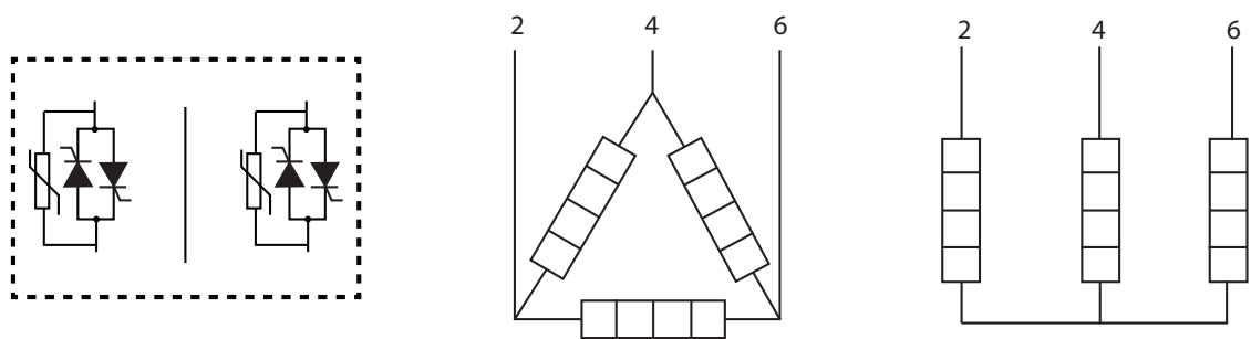
Figure 34 - Three-phase Connections
