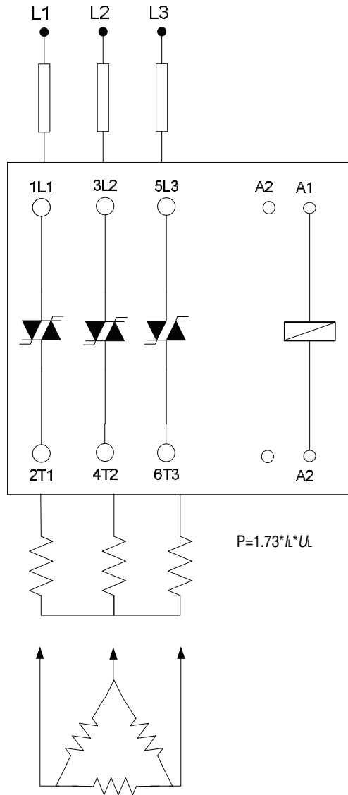
Figure 38 - Three-phase Contactor, Delta and Star Connection
