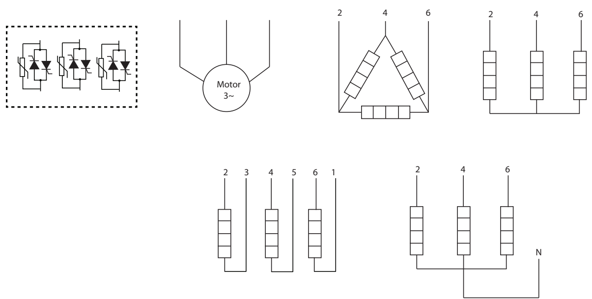
Figure 34 - Three-phase Connections
