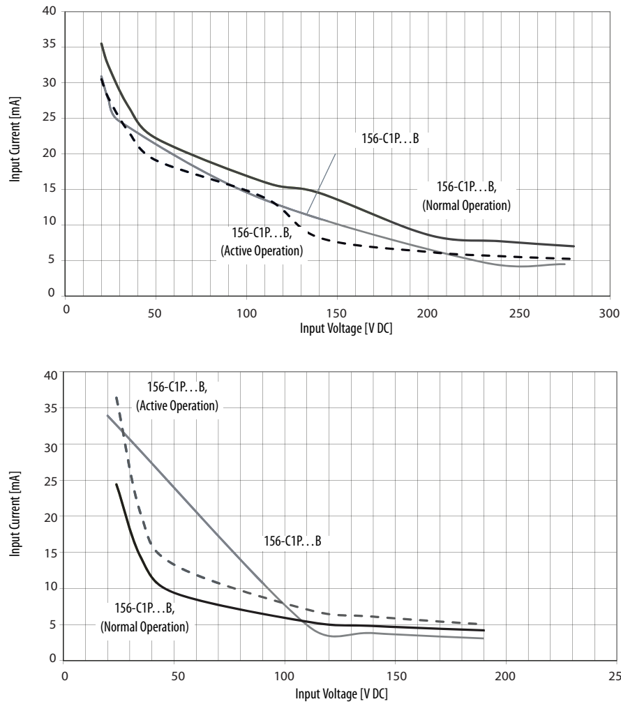
Figure 2 - 156-C1P...B A1 Input Current vs. Input Voltage
