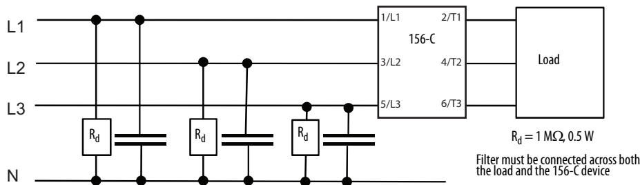
Figure 31 - Terminal Layout
