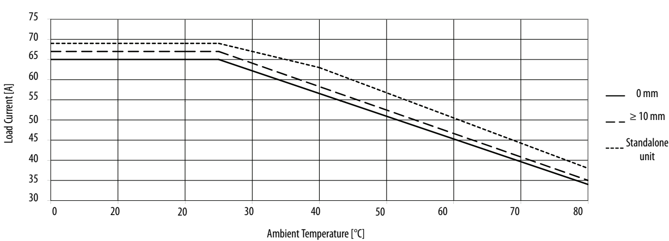
Figure 14 - 156-C1P65 Space Derating
