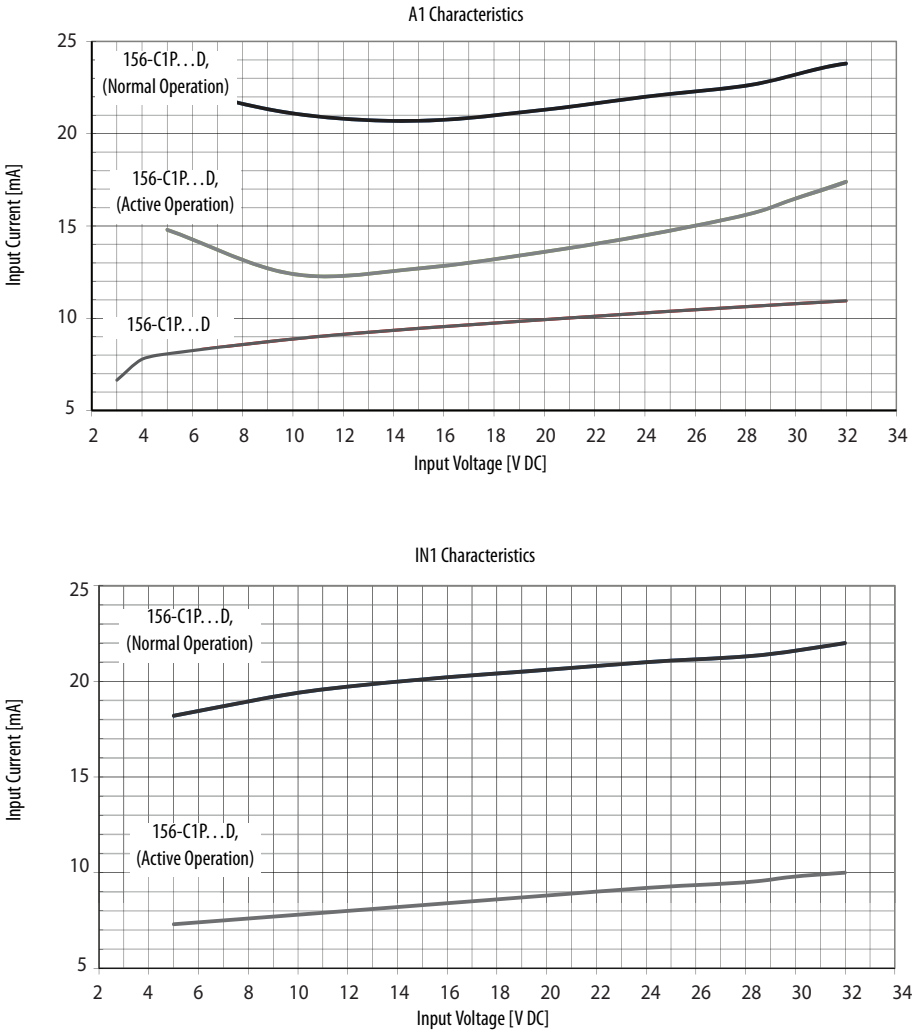
Figure 1 - 156-C1P...D Input Current vs. Input Voltage
