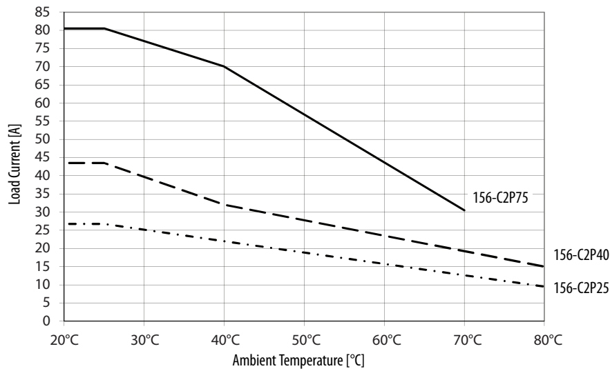
Figure 28 - Dual-phase 0 mm Spacing Temperature Derating
