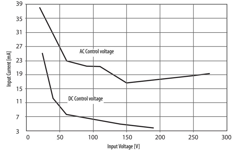
Figure 21 - Cat. No. 156-C...A Input Current vs. Input Voltage
