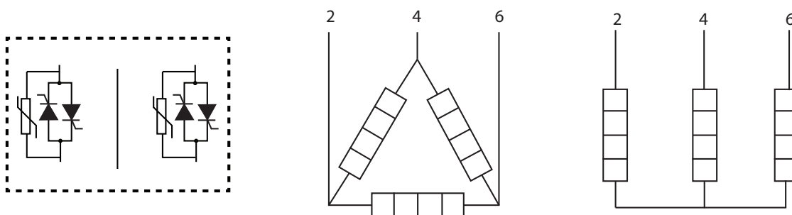
Figure 34 - Three-phase Connections
