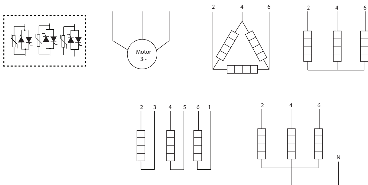
Figure 34 - Three-phase Connections
