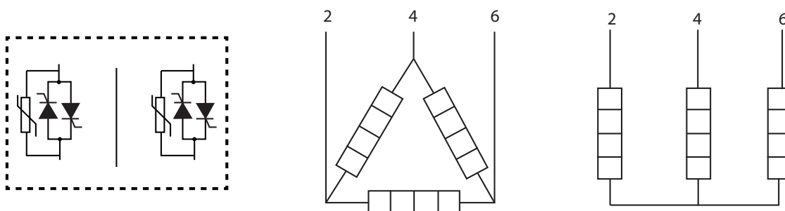
Figure 34 - Three-phase Connections
