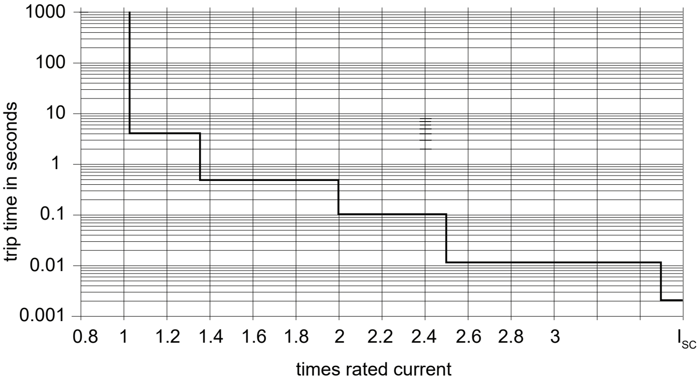
Typical time/current characteristic ( T_{amb} = +23\text{ }^{\circ}\text{C} , UB = DC 24 V)
