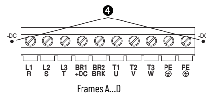
Power Terminals
