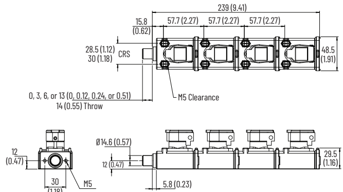
Figure 158 - Quad Key [mm (in.)]
