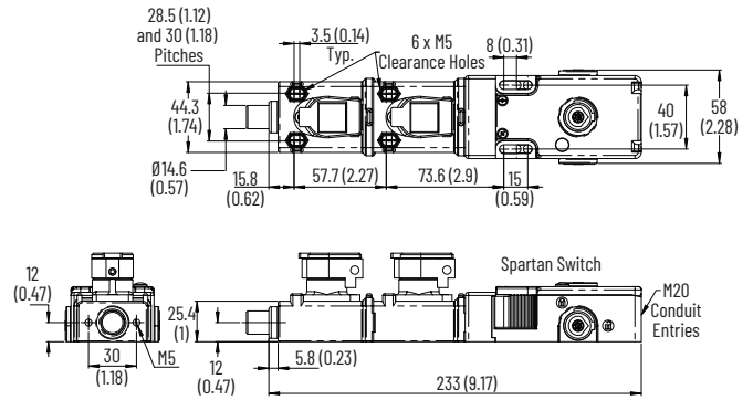
Figure 162 - Prosafe Bolt Lock Solenoid Locked with Electrical Isolation - Two Keys [mm (in.)]
