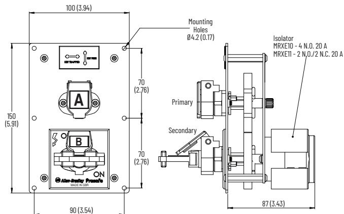
Figure 131 - MRXE10 and MRXE11 [mm (in.)]
