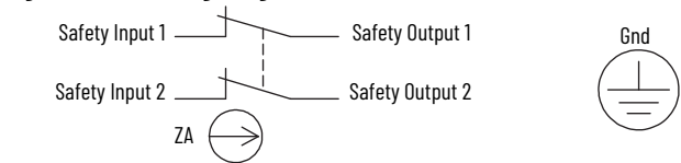
Figure 102 - Wiring Diagram
