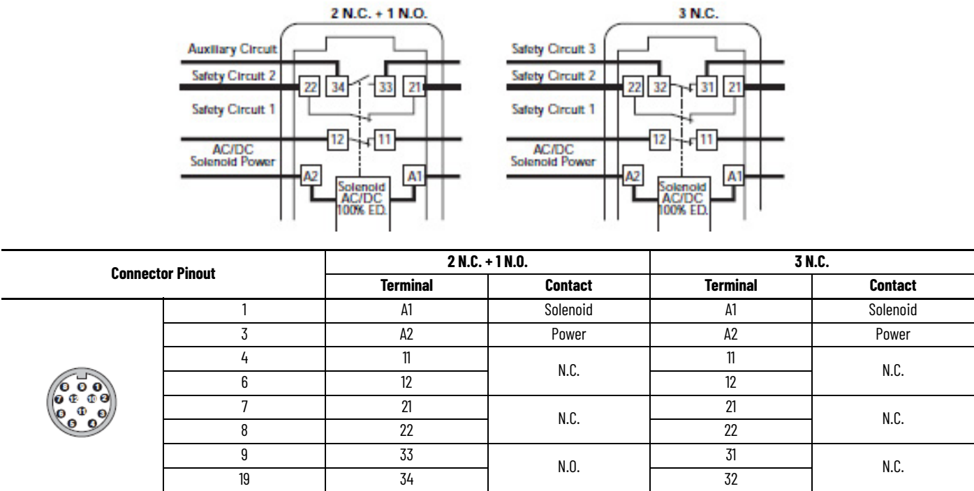
Figure 15 - Contact Action
