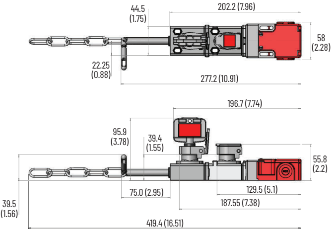
Figure 166 - Electrical, Dual Key, Chain Actuator [mm (in.)]
