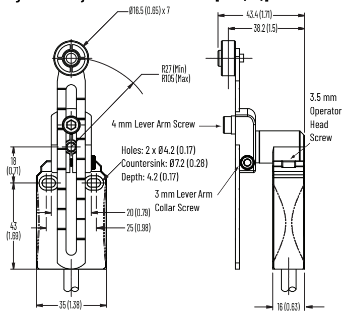
Figure 108 - Adjustable Roller Lever Arm [mm (in.)]
