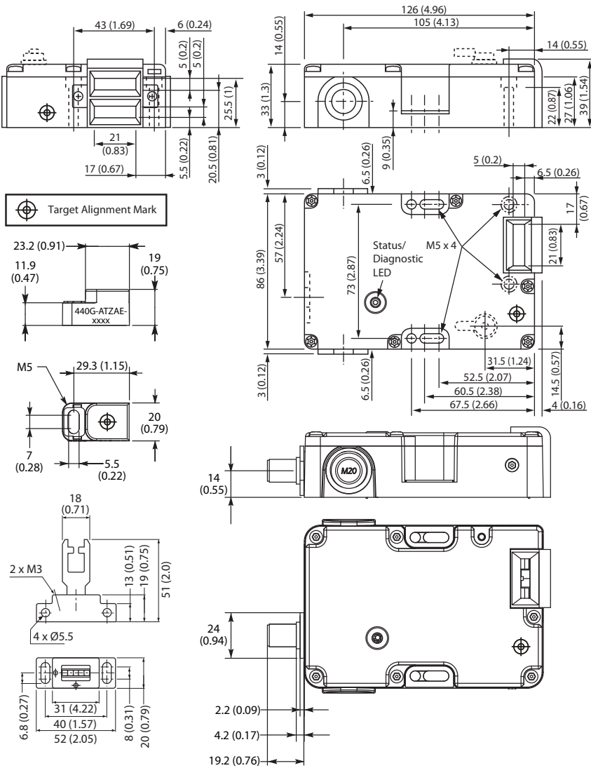
Figure 7 - Guard Locking Switch [mm (in.)]
