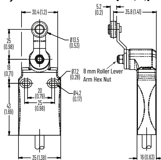
Figure 108 - Adjustable Roller Lever Arm [mm (in.)]
