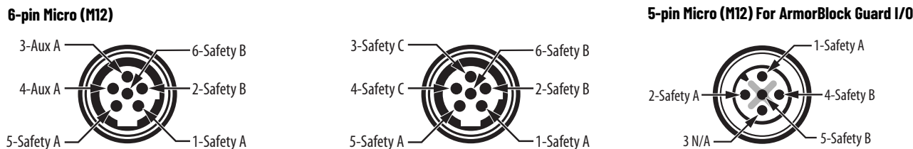
Figure 25 - Connections
