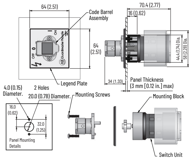
Figure 136 - RPSE10 and RPSE11 [mm (in.)]
