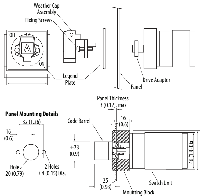
Figure 138 - RPSE16 [mm (in.)]
