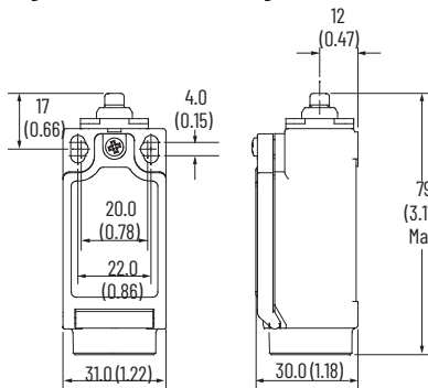
Figure 113 - Hinge Lever [mm (in.)]
