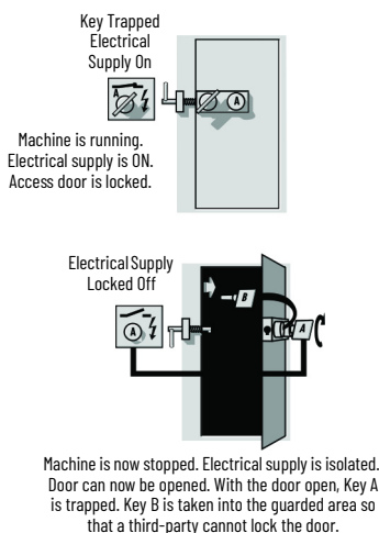
Figure 128 - Full Body Access
