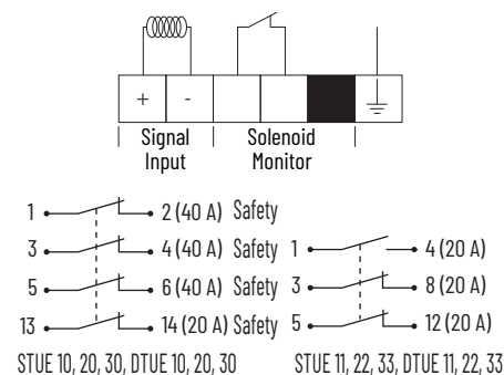
Figure 149 - Wiring (Shown with Power On)
