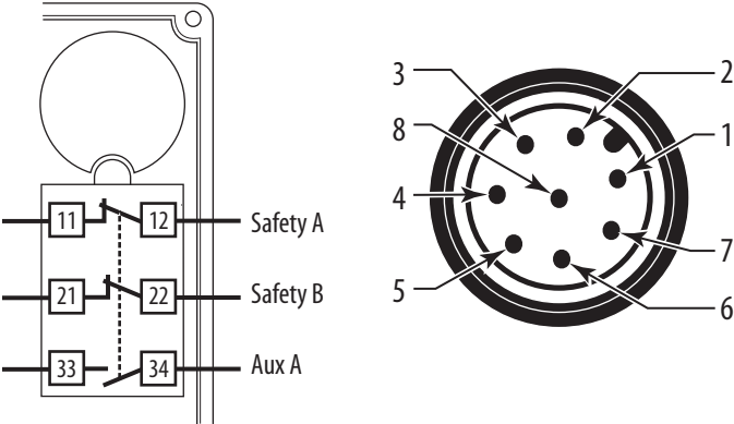
Figure 27 - Contact Configuration 2 N.C. and 1 N.O.
