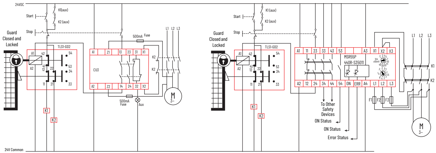
Figure 5 - TLSZ-R Guard Locking Example
