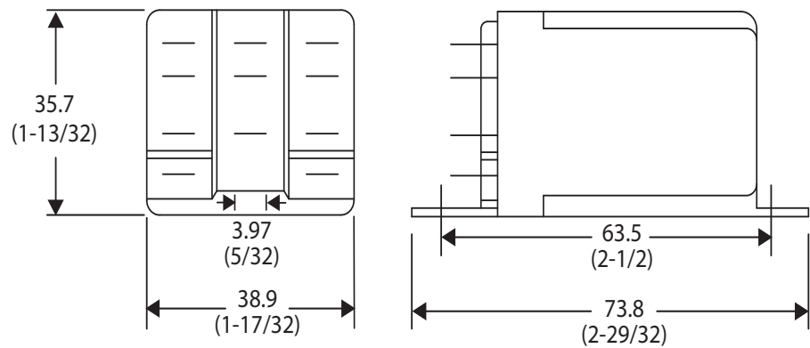
700-HHF Relay
