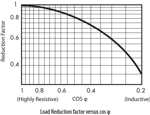
Load Reduction factor versus \cos \phi
