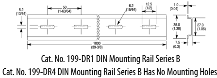
Cat. No. 199-DR4 DIN Mounting Rail Series B Has No Mounting Holes
