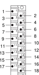
1492-CAB01T64
