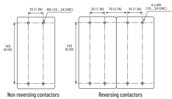
Figure 82 - 100-E265...100-E370 Contactors
