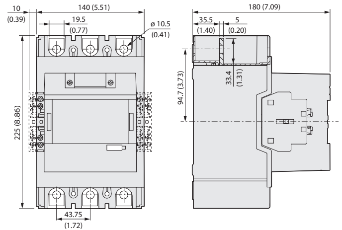
Figure 83 - 100-E265E...100-E370E Contactors with PLC Input
