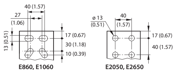
Figure 89 - 100-E860, 100-E1060, 100-E2050, 100-E2650 Contactors with PLC Input
