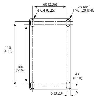
Figure 63 - Drilling Template for 40...52 A 4-Pole Contactors
