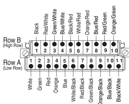
1492-CAB0T64
