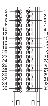
1492-CABLE0TBCH
