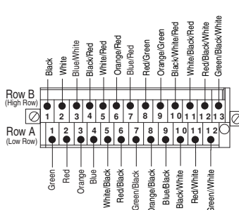
1492-CAB0T64
