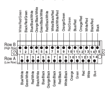
1492-CAB0X62
