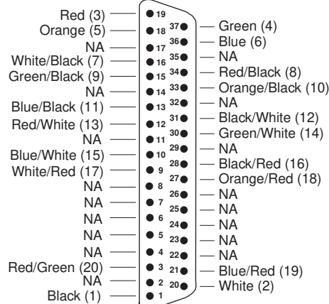
Flex D-shell End 1492-CAB1A94
