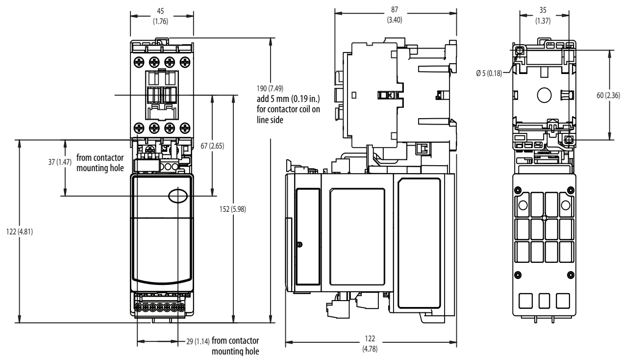
Figure 6 - E300/E200 Overload Relay Mounted on Bulletin 100-C09...-C23 Contactor
