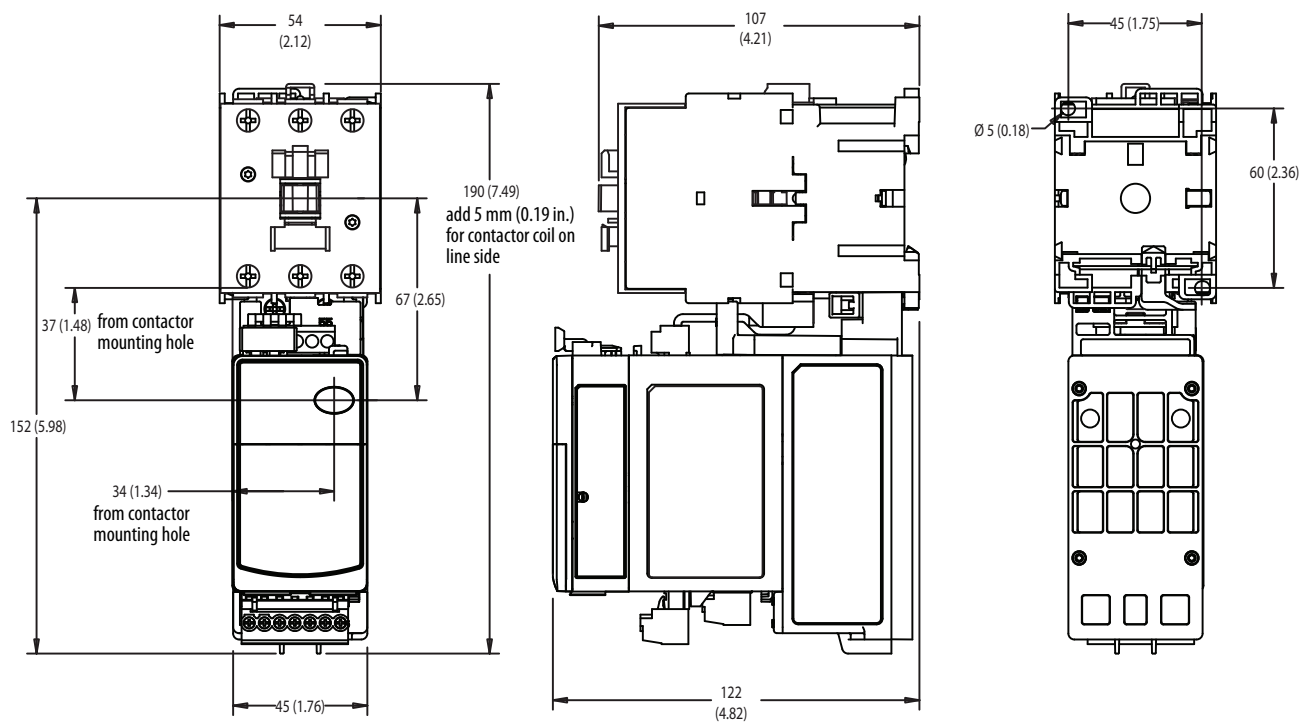
Figure 8 - E300/E200 Overload Relay Mounted on Bulletin 100-C43...-C55 Contactor
