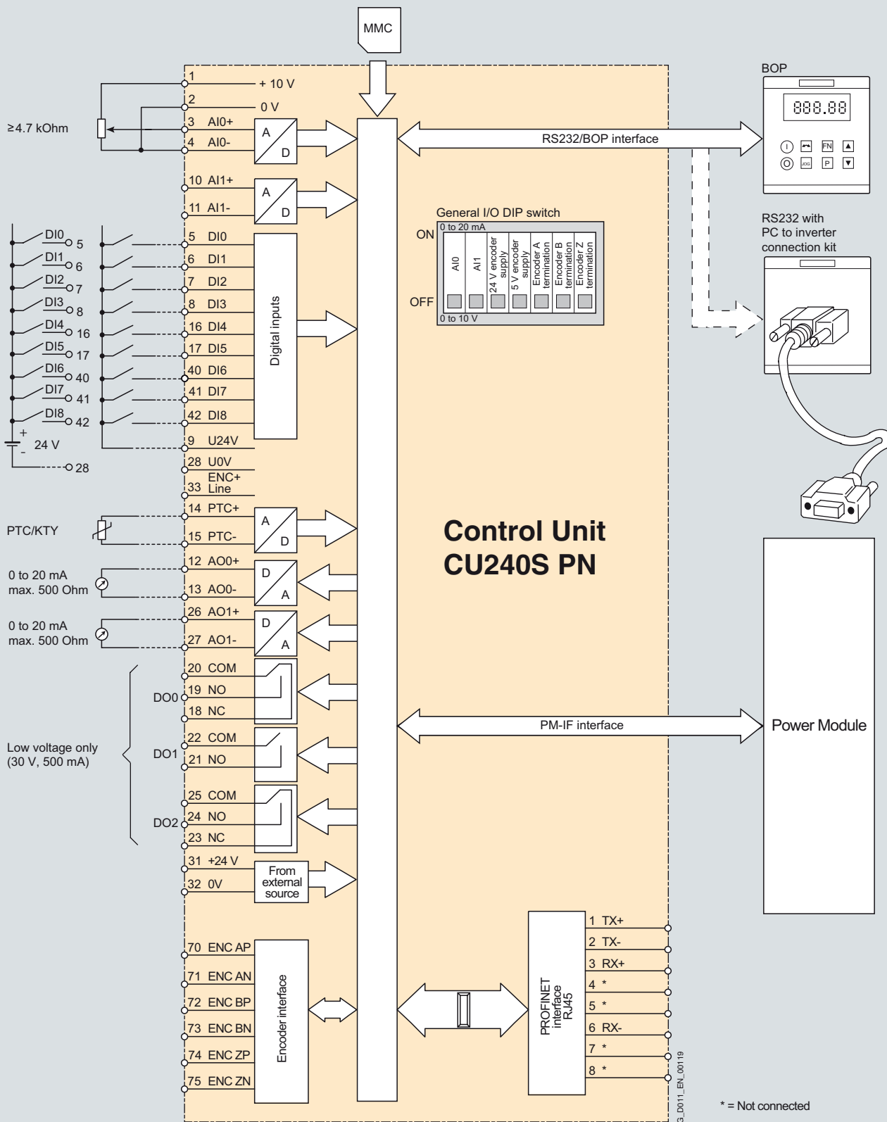
CU240S PN Control Unit connection diagram
